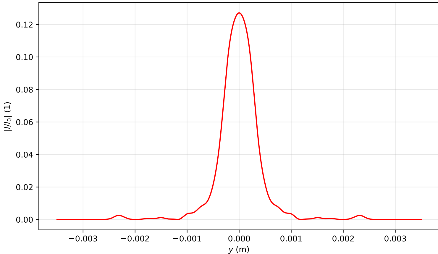
Intensity profile I(x=0, y, z=3.503)/I_0 , P_{in}=6.0P_{cr} , artificial time
